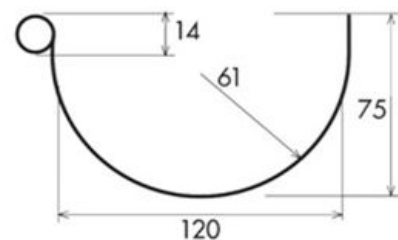
Section GRN125
