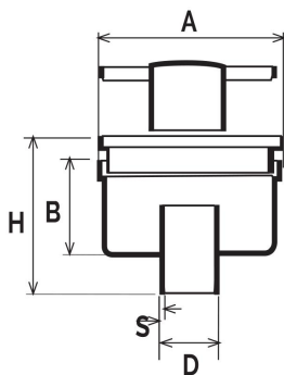
vertical outlet
