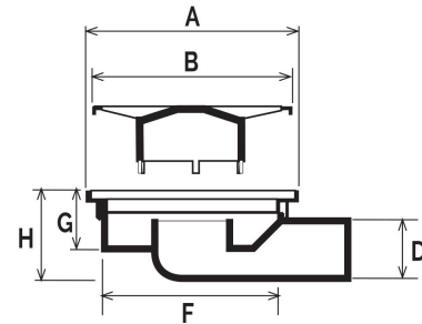
adjustable horizontal outlet
