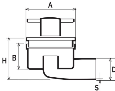
adjustable horizontal outlet
