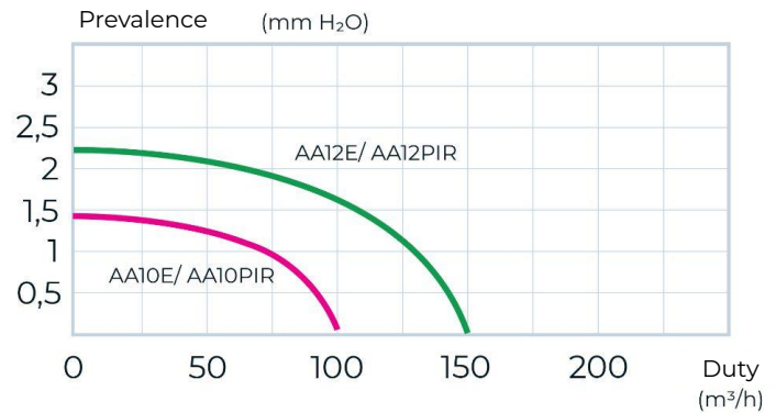
Flow rate curve
